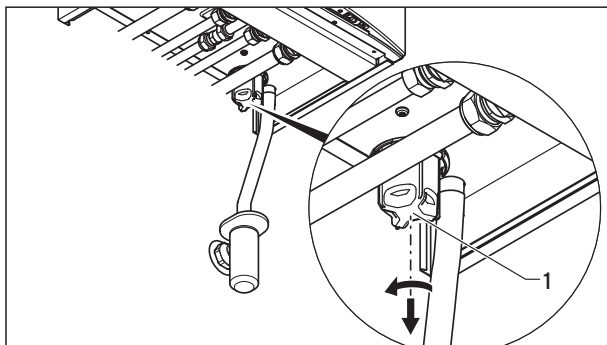
Afb. 8.11 Condenswatersifon reinigen
